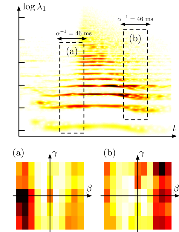
Figure 3: Top: scalogram of a musical note from Berio's Sequenza V for trombone, around 3'45". Observe that the attack part (a) has increasing pitch and increasing brightness, whereas the release part (b) has decreasing pitch and decreasing brightness. Bottom: spiral scattering coefficients for t and \log \lambda_1 specified by (a) and (b), \alpha^{-1} fixed at 46 ms, \beta^{-1} ranging from -1 octave to +1 octave, and \gamma^{-1} ranging from -4 octaves to +1 octaves. As expected, highest values are concentrated in the bottom left corner for (a) and in the top right corner for (b).
